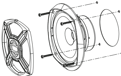
TYPICAL MOUNTING
